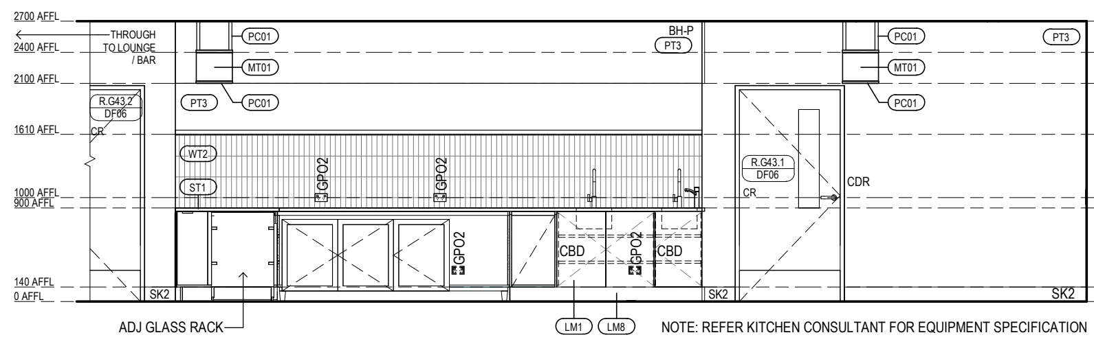
VILLAGE LIFESTYLE - CAFE AREA ELEVATION 3 Scale 1 : 50
