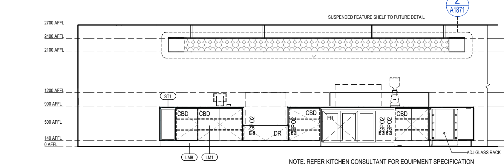
VILLAGE LIFESTYLE - CAFE AREA ELEVATION 1 Scale 1 : 50
