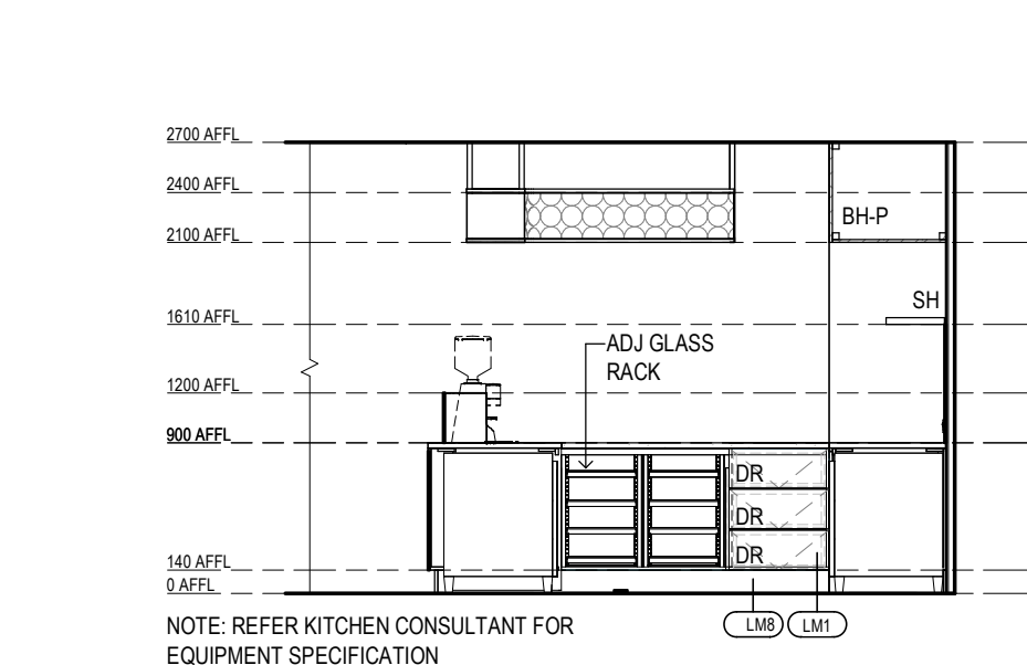
VILLAGE LIFESTYLE - CAFE AREA ELEVATION 2 Scale 1 : 50
